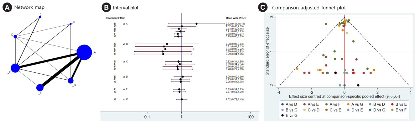
Supplementary Fig. 11. (A) Network map, (B) interval plot, and (C) comparison-adjusted funnel plot for network meta-analysis of antidiabetic drugs on total stroke among subjects with baseline glycosylated hemoglobin \geq average 8.0% ( n=51 trials). The global test for inconsistency gives a P value of 0.918, giving no evidence of inconsistency. A, placebo; B, metformin; C, sulfonyl-urea; D, thiazolidinedione; E, dipeptidyl peptidase-4 inhibitor; F, sodium glucose cotransporter-2 inhibitor; G, glucagon-like peptide-1 agonist; CI, confidence interval.
