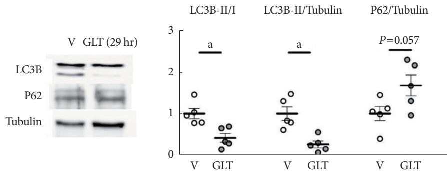
Supplementary Fig. 4. Autophagy activity in mouse islets under chronic glucolipotoxicity (GLT). Mouse islets were exposed to GLT (glucose 20 mM and palmitate 0.5 mM) for 29 hours, total protein was extracted, and Western blotting was performed. Experiment numbers 5 to 6. The lines and error bars represent mean \pm standard error of the mean. Student's t -test was applied. V, vehicle; LC3B, light chain 3B. a P < 0.01.
