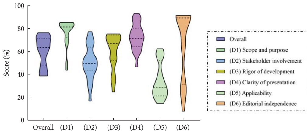
Supplementary Fig. 2. The distribution of scores in the overall and six domains.
